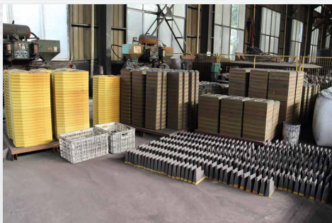
Sand Core Making
