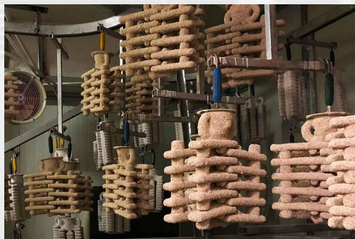
Shell Drying
