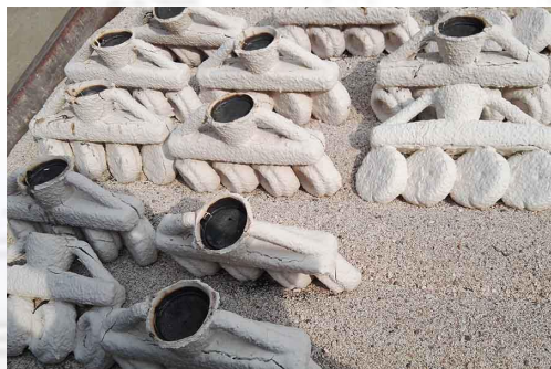
Shell Mold
